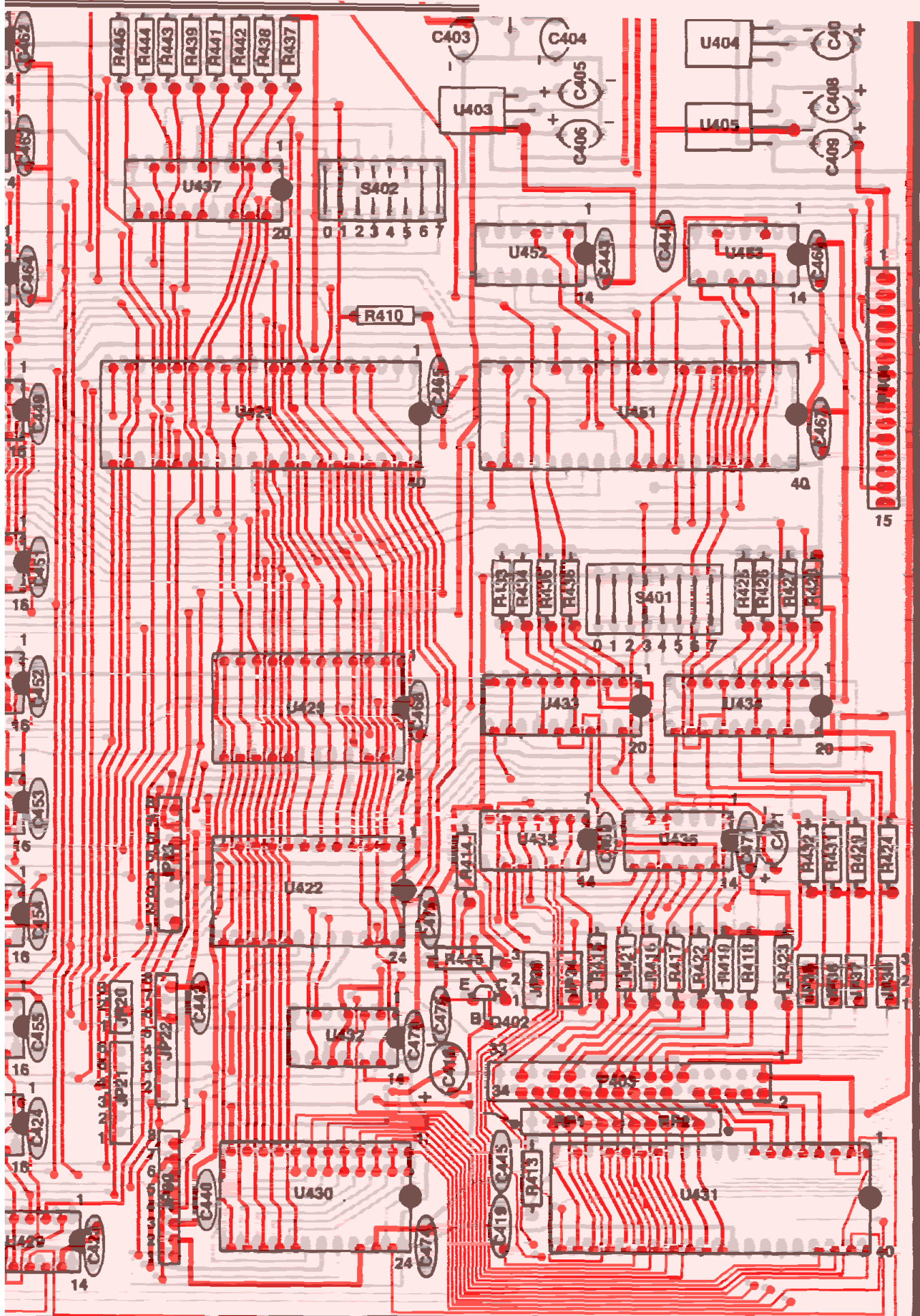
CIRCUIT BOARD (component side)
