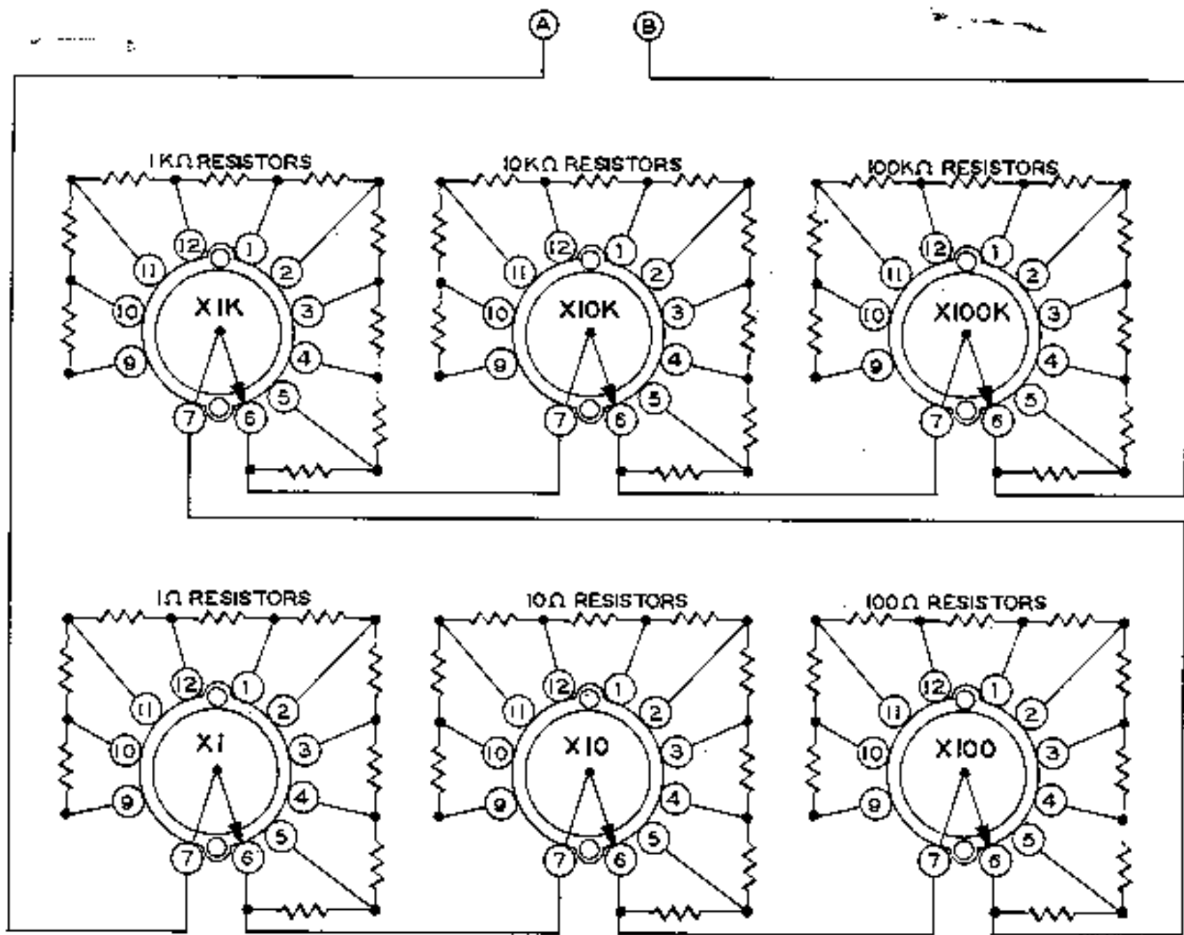
SCHEMATIC DIAGRAM MODEL IN-11
