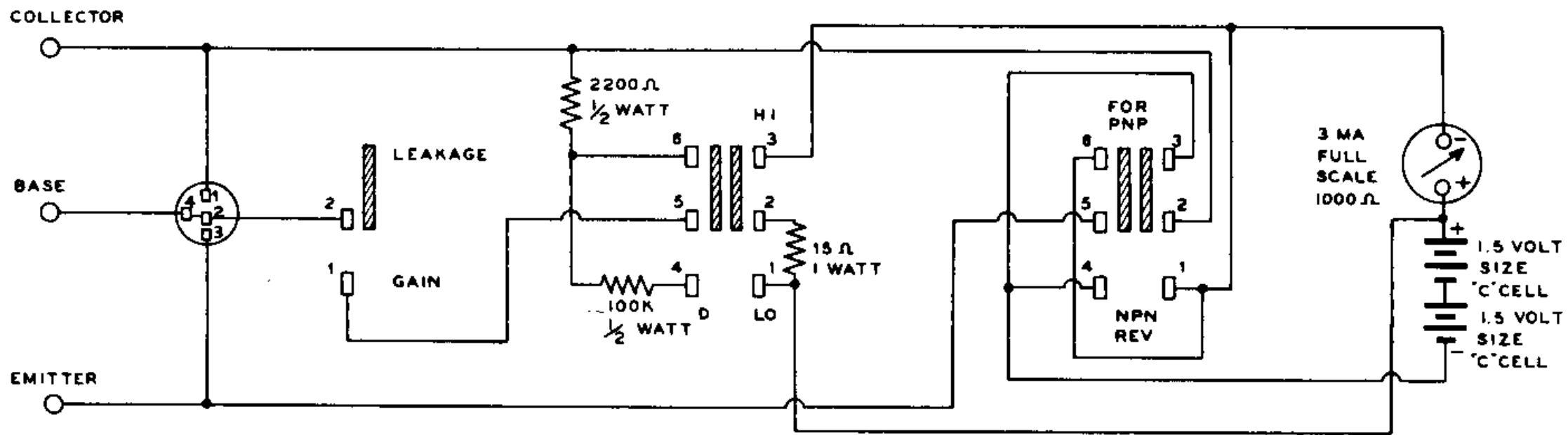
SCHMATIC DIAGRAM
