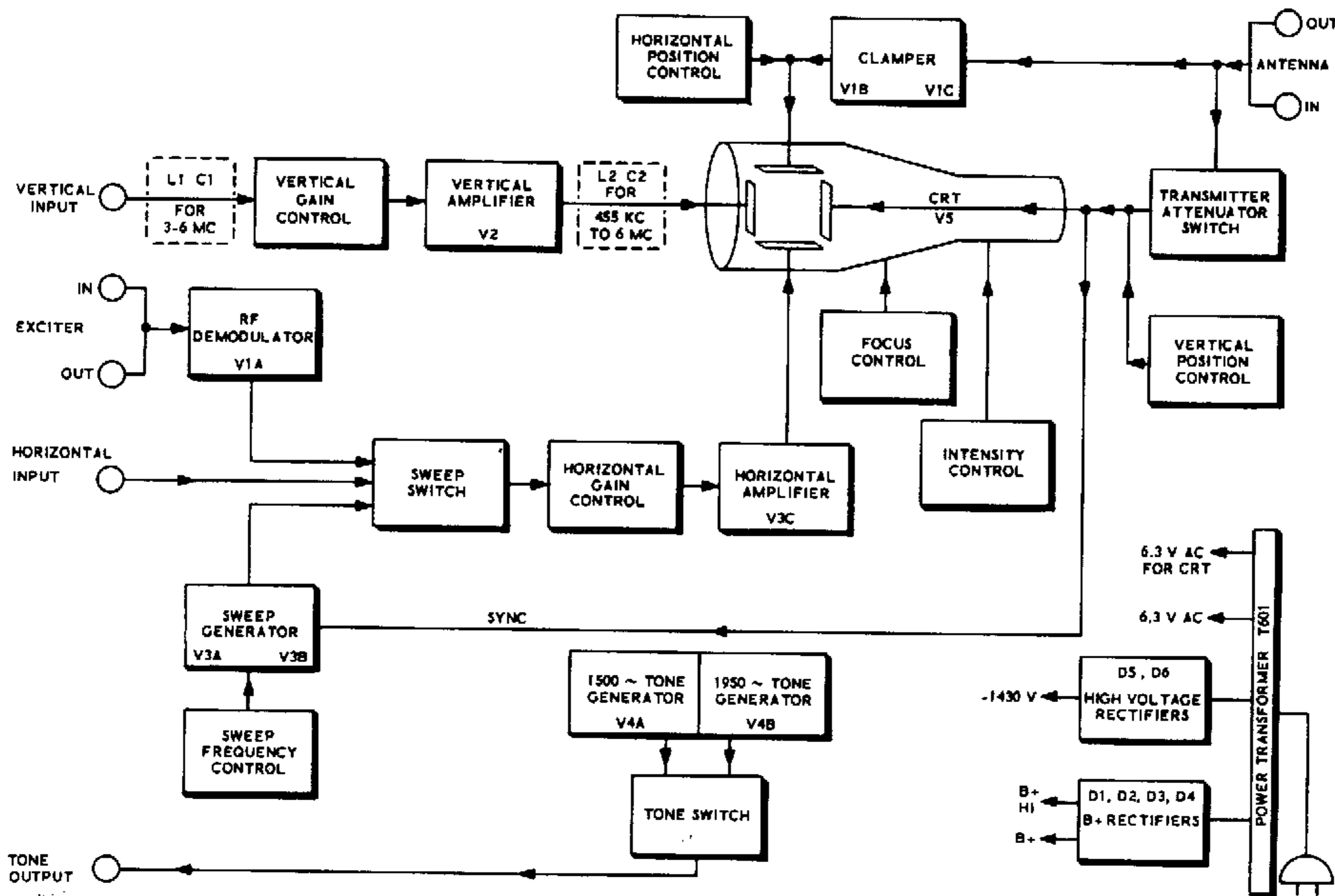
BLOCK DIAGRAM
