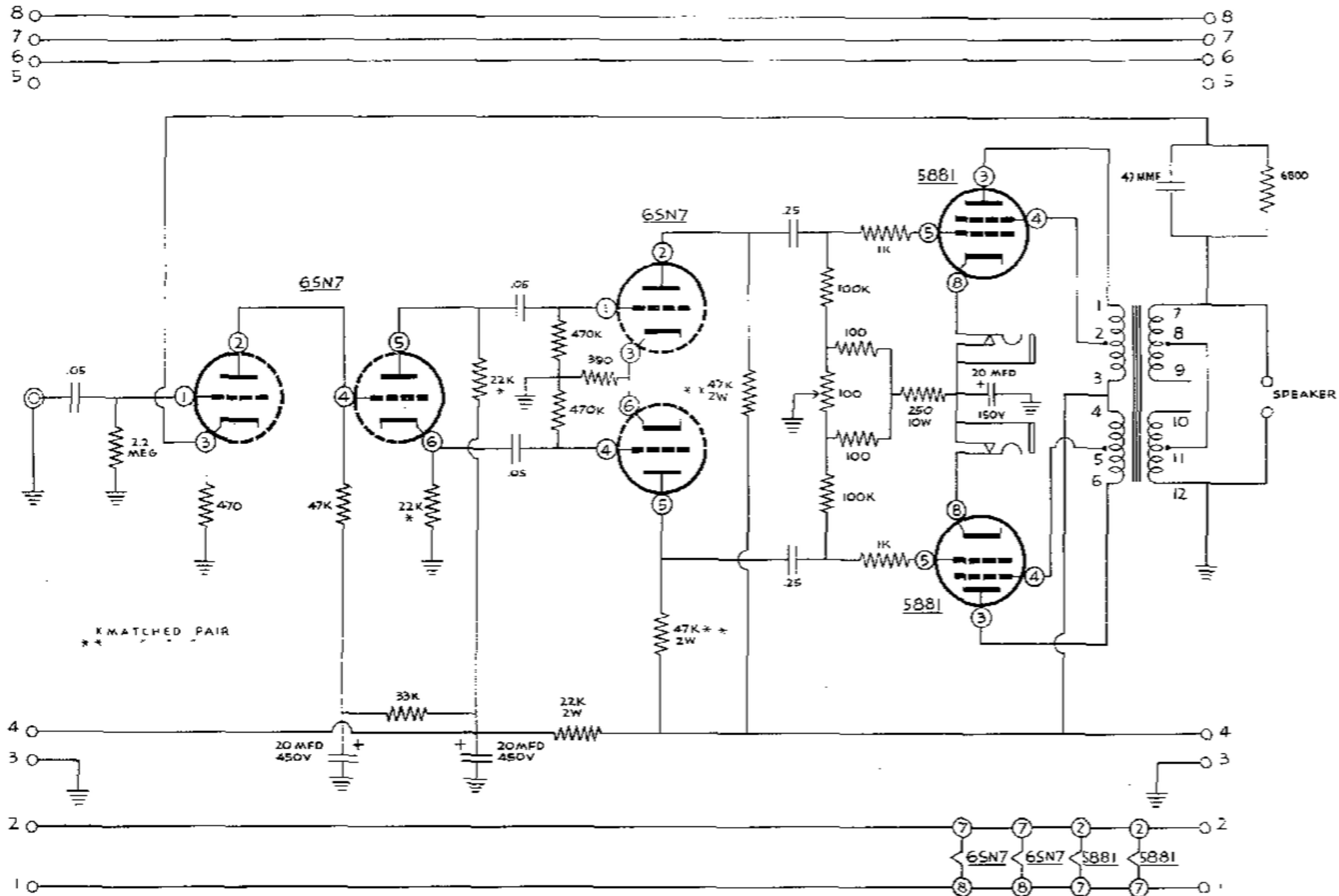
Heathkit MODEL W-2 AMPLIFIER CIRCUIT DIAGRAM
