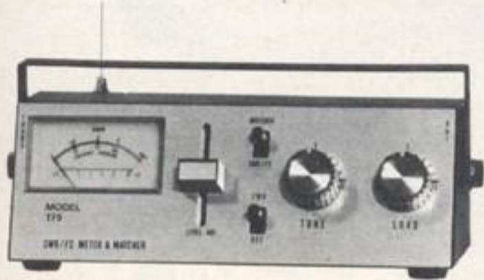
MODEL 175 3-Function CB/HAM Tester
