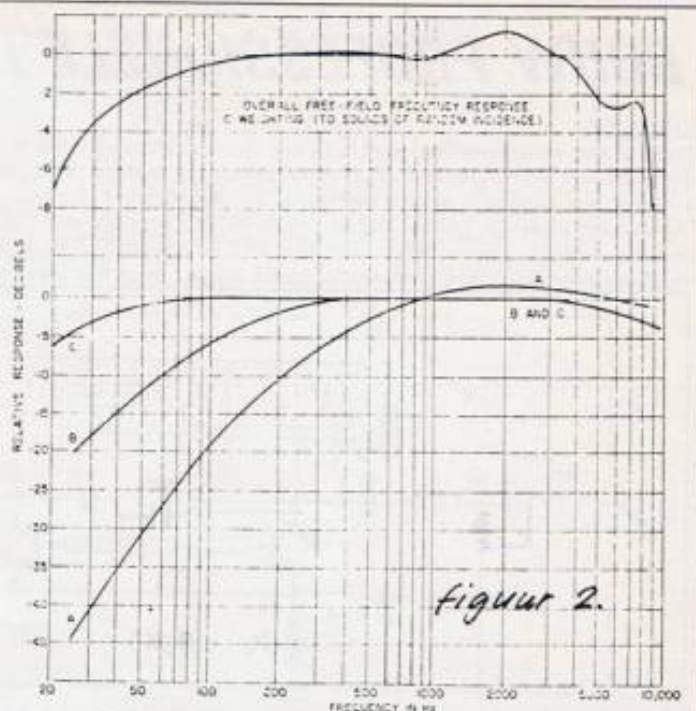
USASI (ASA) Standard S1.4-1961. Weighted curves for sound-level meters. Used in all instruments manufactured since 1951.
