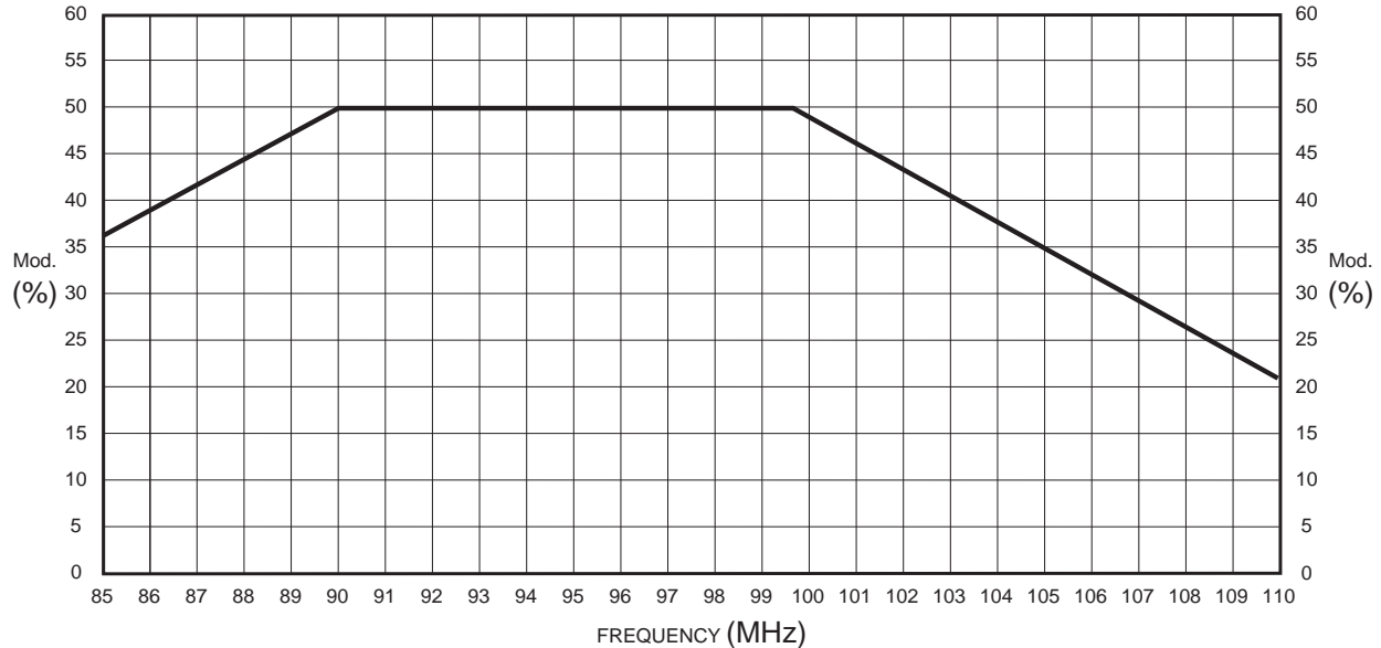
Illustration 2-9 Modulation Compensator Settings
