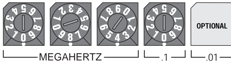
Illustration 2-7 RF Exciter Board (Frequency Selector Switches)
