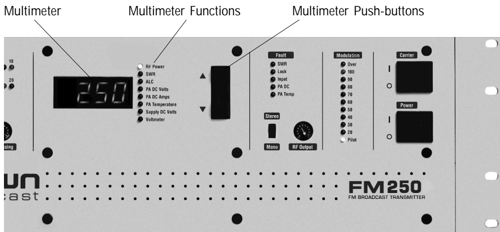
Illustration 3-5 Digital Multimeter
