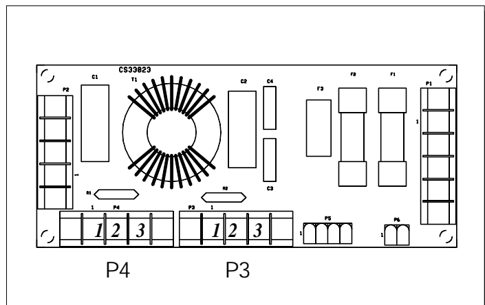
NA 501: Positioning of the power supply internal terminal board
