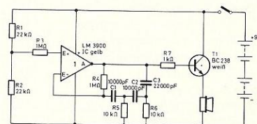
Afb. 2. Schema toongenerator
